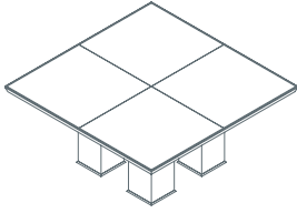
Meeting table, with square base and top 1IA4011: L 63 D 63 H 28¼
